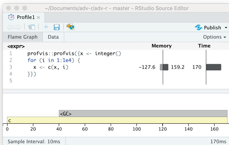
Figure 23.4 Profiling a loop that modifies an existing variable reveals that most time is spent in the garbage collector (<GC>).
