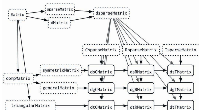
Figure 16.1 A small subset of the Matrix class graph showing the inheritance of sparse matrices. Each concrete class inherits from two virtual parents: one that describes how the data is stored (C = column oriented, R = row oriented, T = tagged) and one that describes any restriction on the matrix (s = symmetric, t = triangle, g = general).
